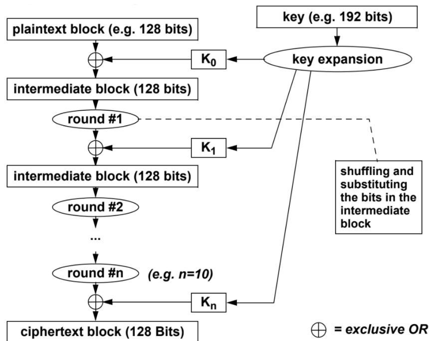
Figure 16, [F16]: Steps of AES Encryption
