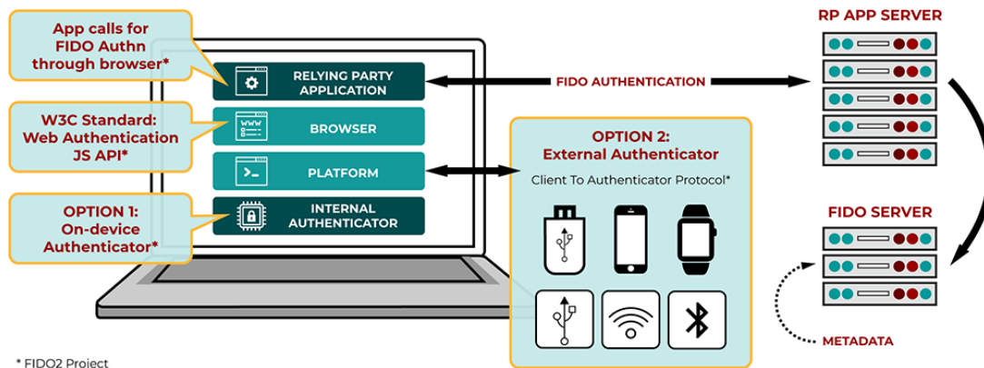
Figure 31, [F31]: CTAP authentication overview
