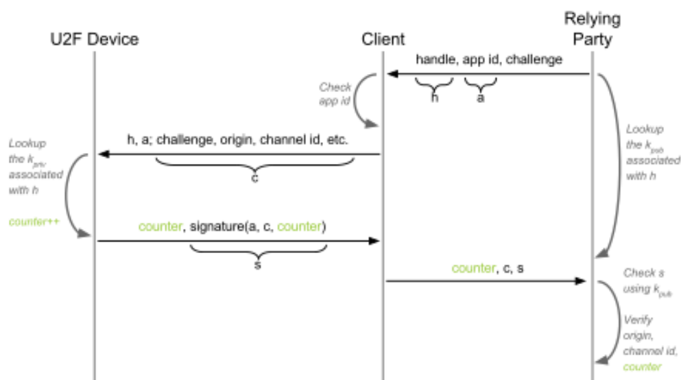
Figure 29, [F29]: FIDO U2F authentication workflow
