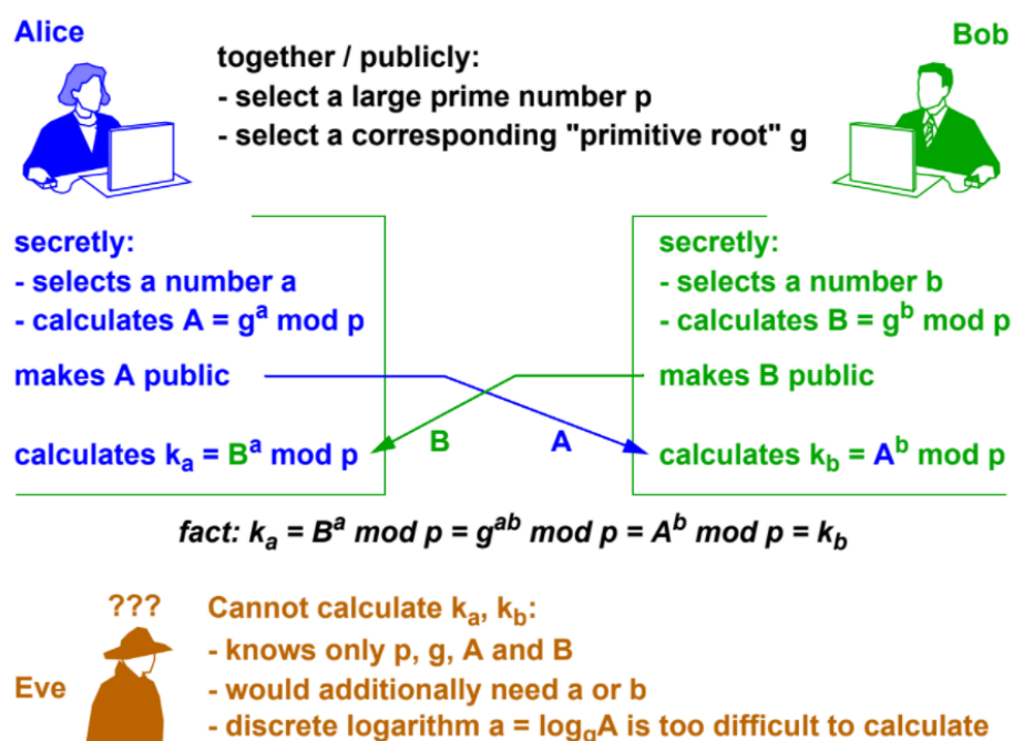
Figure 25, [F25]: The Steps of the Diffie-Hellman Protocol
