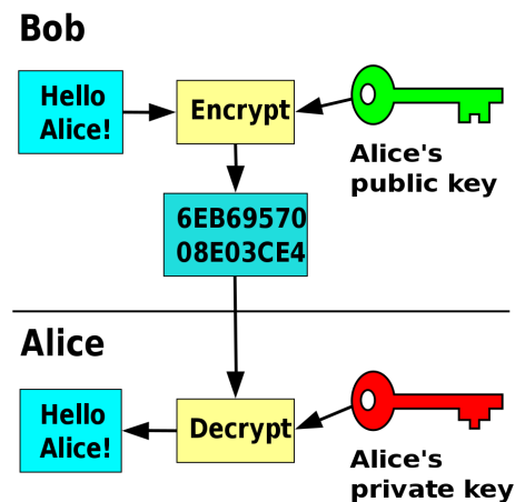
Figure 17, [F17]: Public-Key Cryptography whereas Alice represents the receiver and Bob the sender
