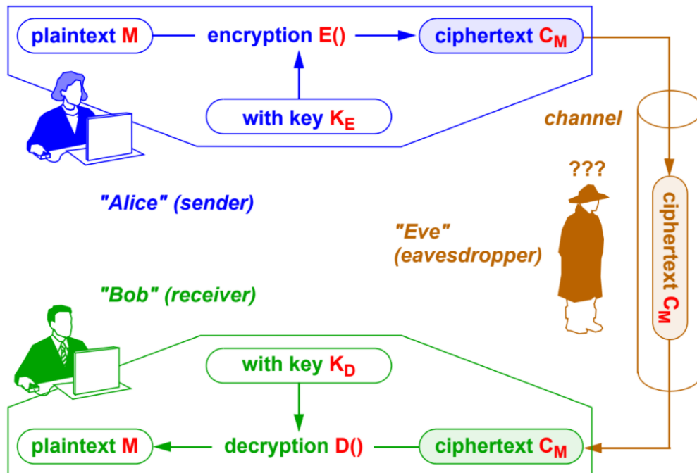
Figure 15, [F15]: Fundamental Model visualized
