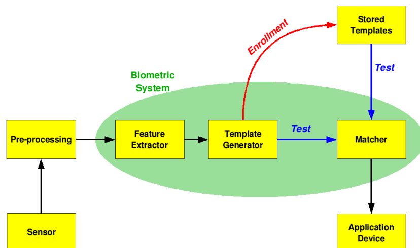
Figure 13, [F13]: Main logical block of a biometric system simplified
