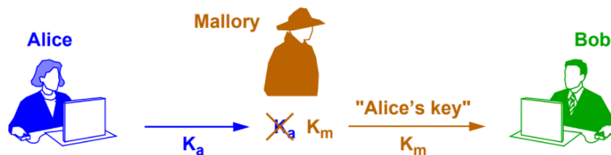
Figure 26, [F26]: Man-in-the-middle attack visualized
