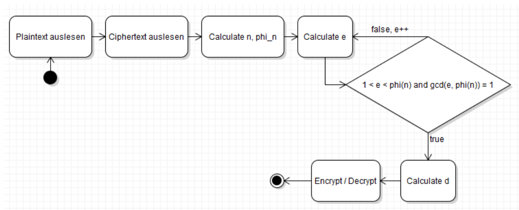
Figure 36, [F36]: Raven One SimuLink RSA uml type activity diagram
