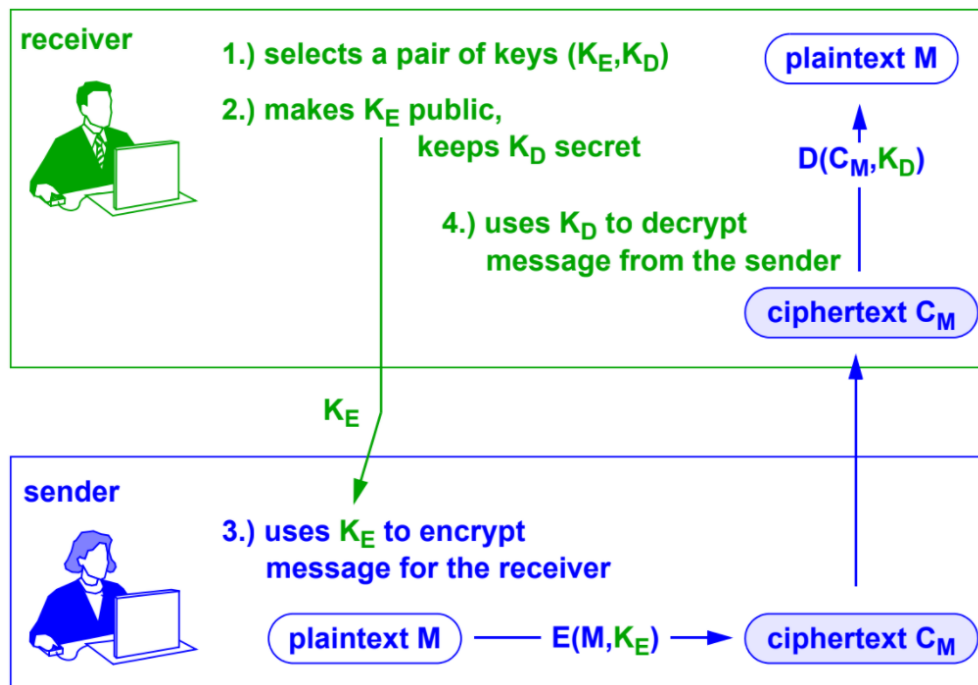
Figure 18, [F18]: Public-Key — The General Model
