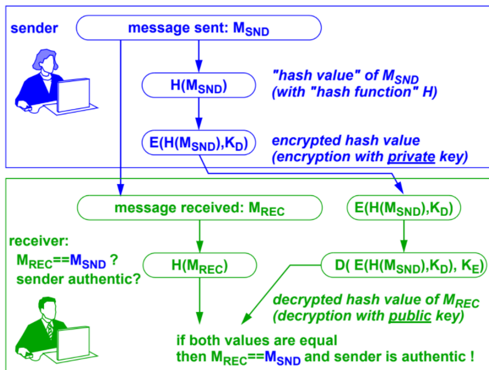
Figure 21, [F21]: Digital Signature: Steps
