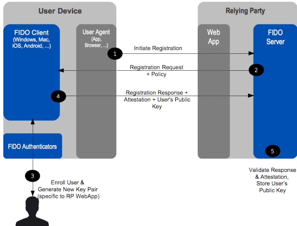
Figure 30, [F30]: FIDO UAF registration message flow
