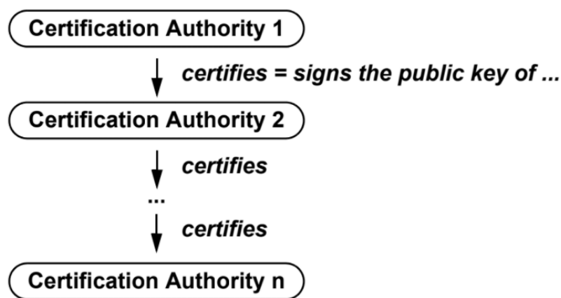
Figure 28, [F28]: Hierarchy of Certification Authorities
